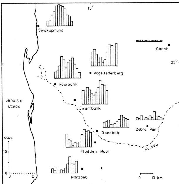
FIGURE 9: Mean monthly number of days with fog-water precipitation.
