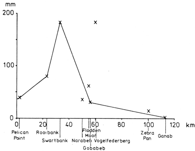
FIGURE 12: Mean annual fog-water precipitation in the central Namib plotted against distance from coast. Values for longer term stations are connected while shorter term stations are indicated by (x) only.
