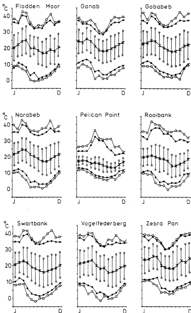
FIGURE 14: Annual march of temperature for all stations. Included are absolute maximum and minimum ( \square - \square ), mean monthly maximum and minimum ( \bullet - \bullet ), mean daily maximum and minimum connected by vertical bar ( \circ - \circ ) and mean daily temperature ( \times - \times ).
