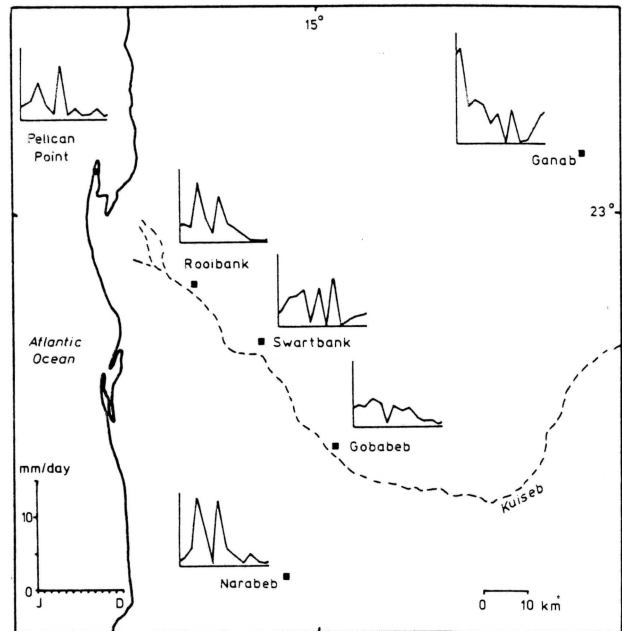
FIGURE 7: Mean rainfall per rain day calculated by month for longer term stations.
