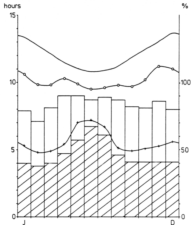
FIGURE 21: Comparison between mean monthly hours of sunshine at Gobabeb (O—O) and Pelican Point (+—+). The top-most curve represents the total number of possible hours sunshine. The histogram indicates percentage of possible sunshine recorded, with Pelican Point shaded.
