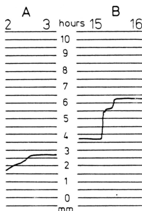
FIGURE 2: Rain gauge chart showing difference in trace between fog (A) and rain (B).
