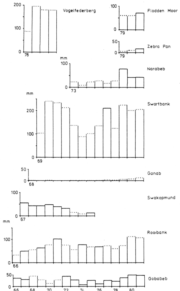
FIGURE 13: Annual total of fog-water precipitation per year. Where the top line of the histogram has been replaced by . . . data are missing for that year.
