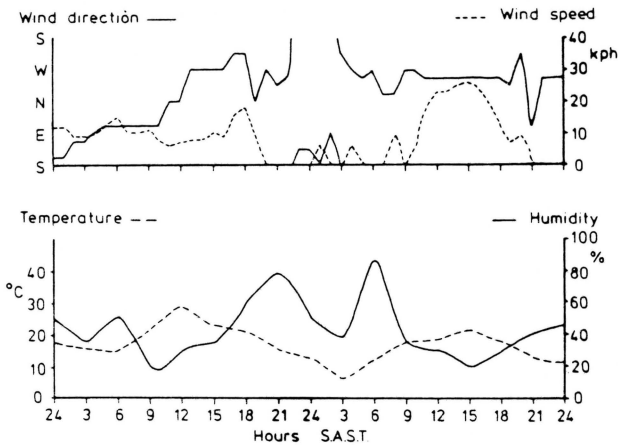
FIGURE 38: Climatic conditions on 13 and 14 September 1979 at Ganab during a fog event in the central Namib. No fog-water precipitation occurred so far inland on these days.
