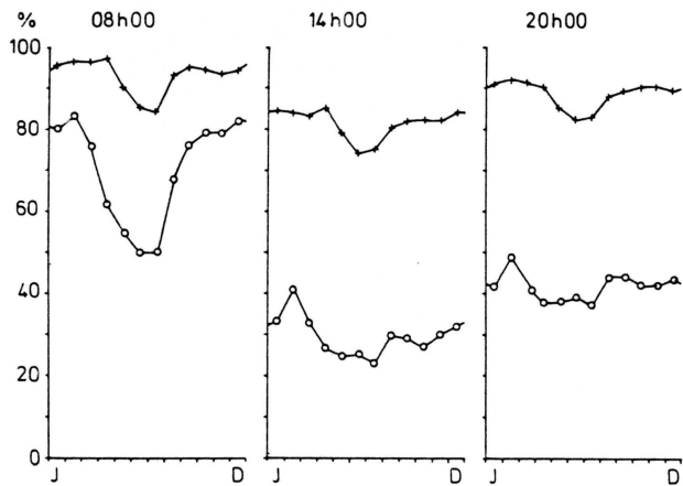
FIGURE 16: Comparison of calculated relative humidity between Pelican Point (+—+) and Gobabeb (○—○) on thrice daily readings from Weather Bureau records.
