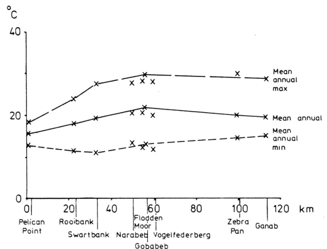
FIGURE 15: Mean annual, mean annual maximum and mean annual minimum temperature for all stations in relation to their distance from the coast. Values for longer term stations are connected while shorter term stations are indicated by (x) only.
