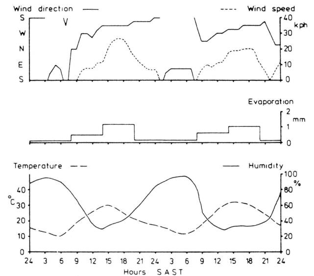
FIGURE 45: Climatic conditions at Gogabeb during 1 and 2 December 1980 with south-westerly wind in the central Namib.
