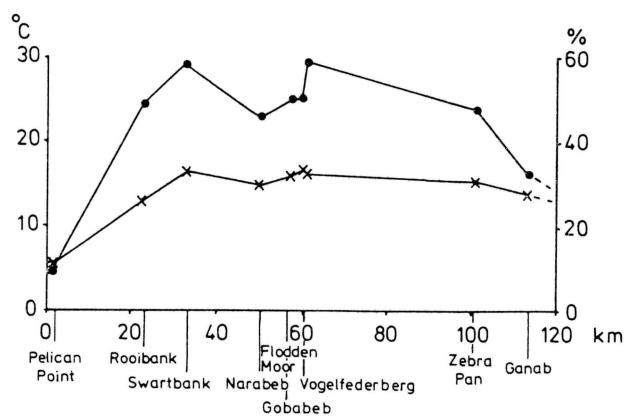
FIGURE 19: Mean annual amplitude of temperature (x—x) and relative humidity (●—●) plotted against distance from the coast.
