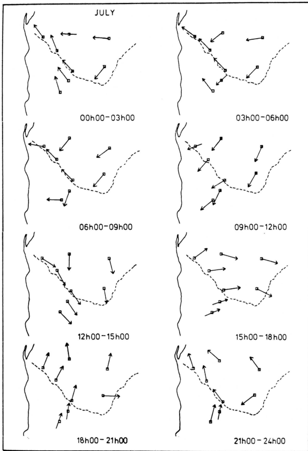
FIGURE 34: Diurnal variation in wind direction for July, as shown by three hourly wind vector directions for Flodden Moor, Ganab, Gobabeb, Narabeb, Swartbank, Rooibank, Vogelfederberg and Zebra Pan.
